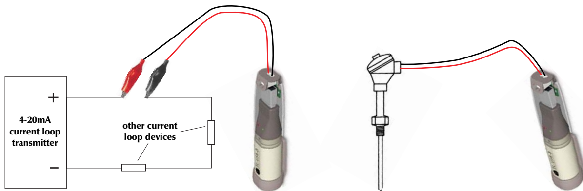
EL-USB-4 fitted to a 4-20mA current loop transmitter
